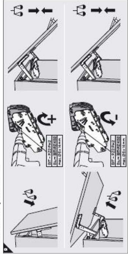
Tension Adjustment
