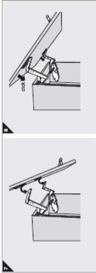
Door Attachment
